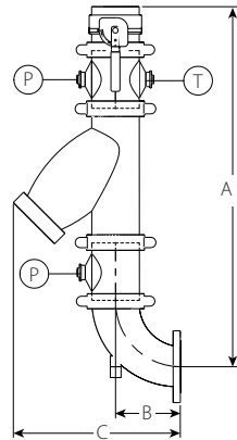
Horizontal Pump Installation
