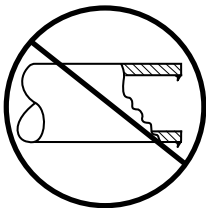
Unacceptable pipe end with burrs
