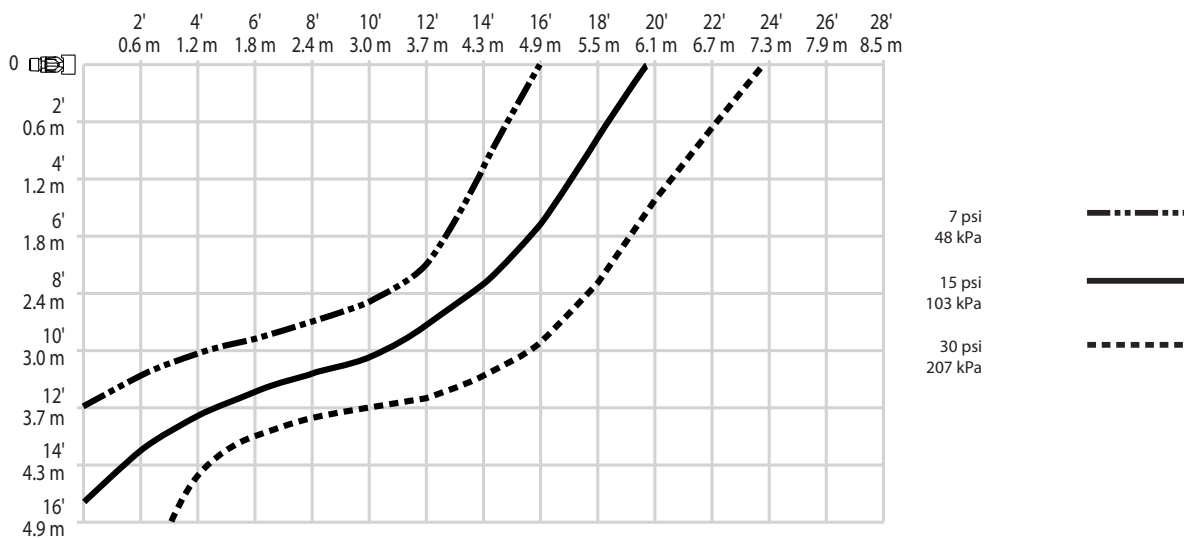
Models V3610, V3609 Horizontal Sidewall and Recessed Horizontal Sidewall Distribution Patterns – Trajectory
