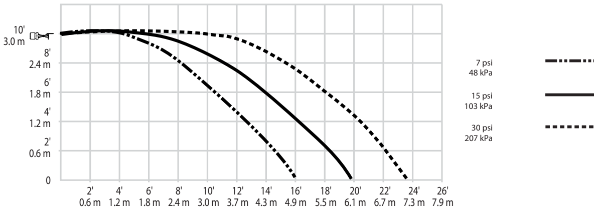
Models V3610, V3609 Horizontal Sidewall and Recessed Horizontal Sidewall Distribution Patterns – Trajectory
